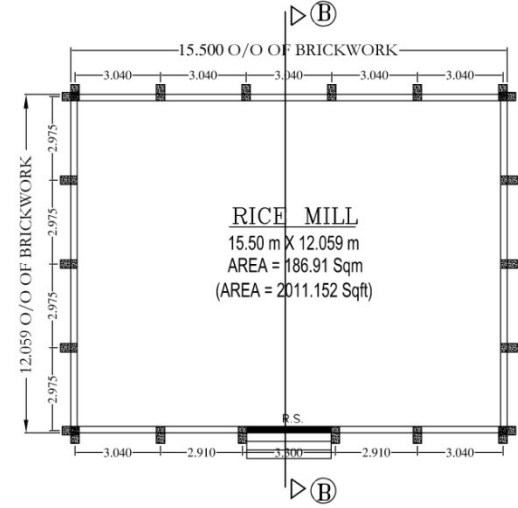
PLAN FOR RICE MILL SHED AT ; SEJGAON
