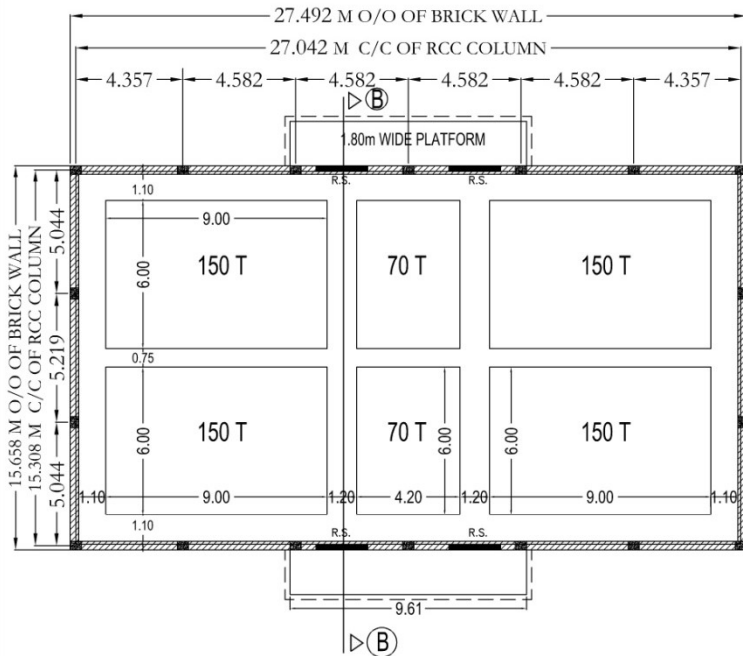
PLAN FOR 1/740 MT.WH. AT ; SEJGAON
